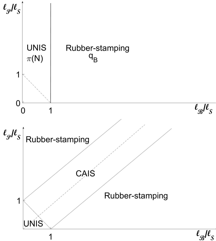
Figure 2: Parameter space with Pareto-efficient symmetric equilibria. Upper panel: without a PA; lower panel: with a PA
