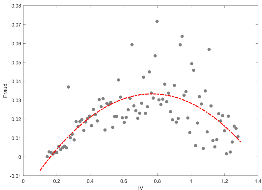
Figure 6: Plot of FRAUD against IV with prediction curve
