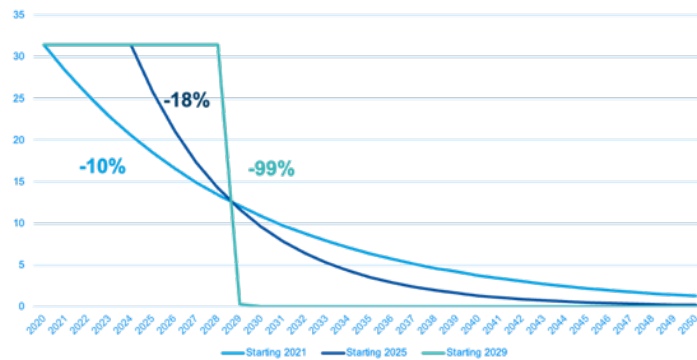
Figure 5: Impact of starting date on carbon pathways
