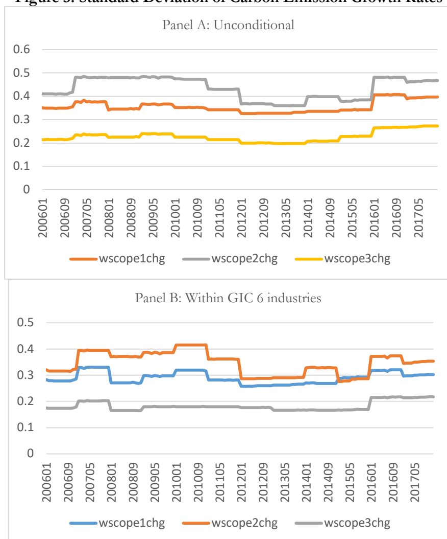
Figure 3. Standard Deviation of Carbon Emission Growth Rates
