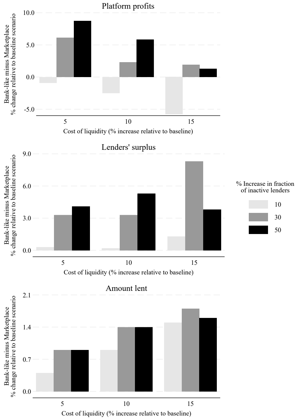
FIGURE 3. SENSITIVITY ANALYSIS
