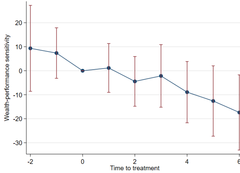
Figure 3: Impact of ISS opposing a stock plan on firms' wealth-performance sensitivity
