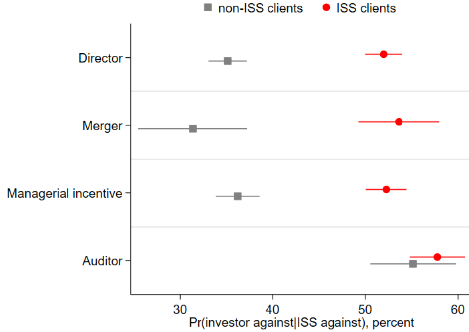
Figure 6: ISS' coordination of investors
